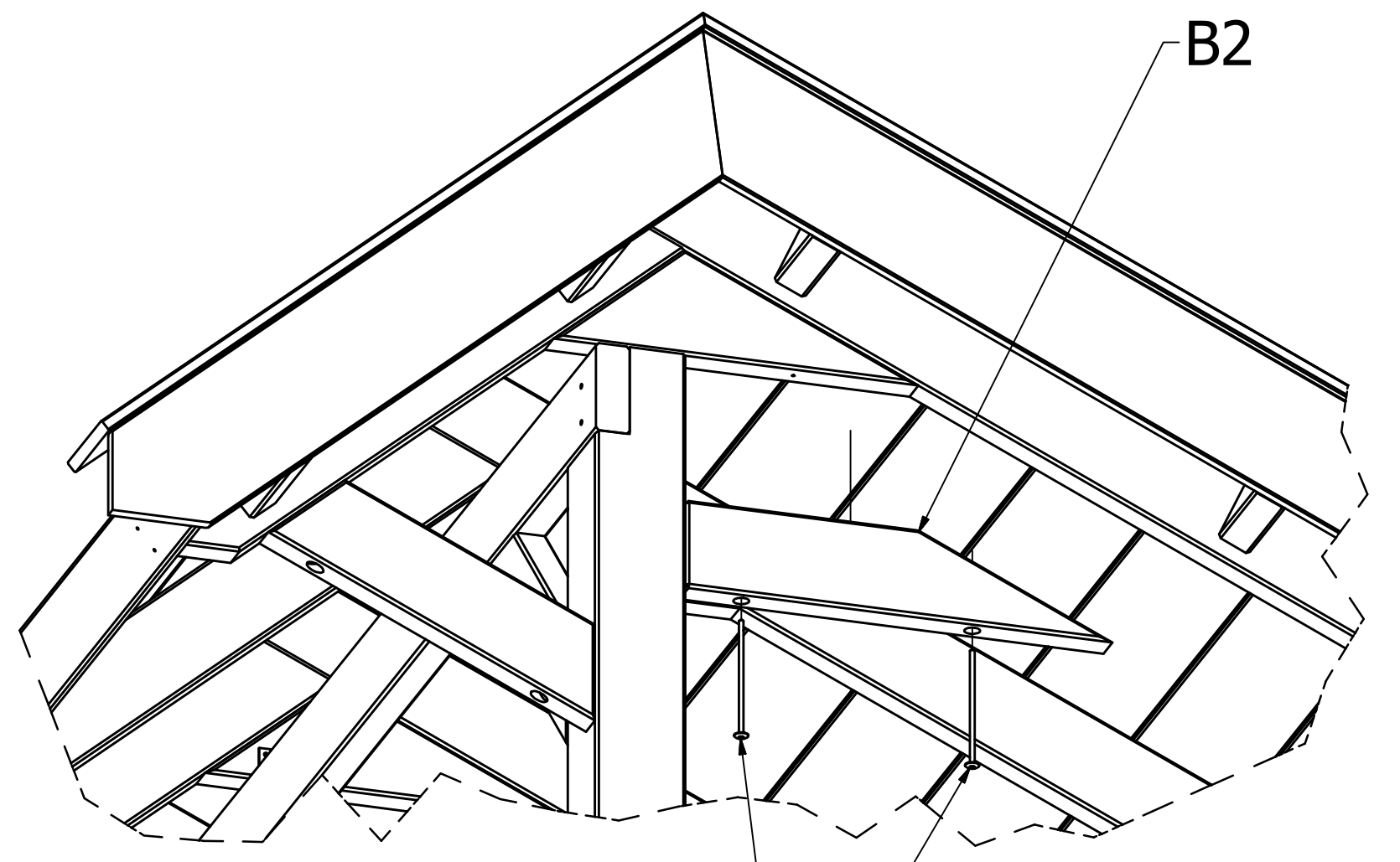
Detail T
